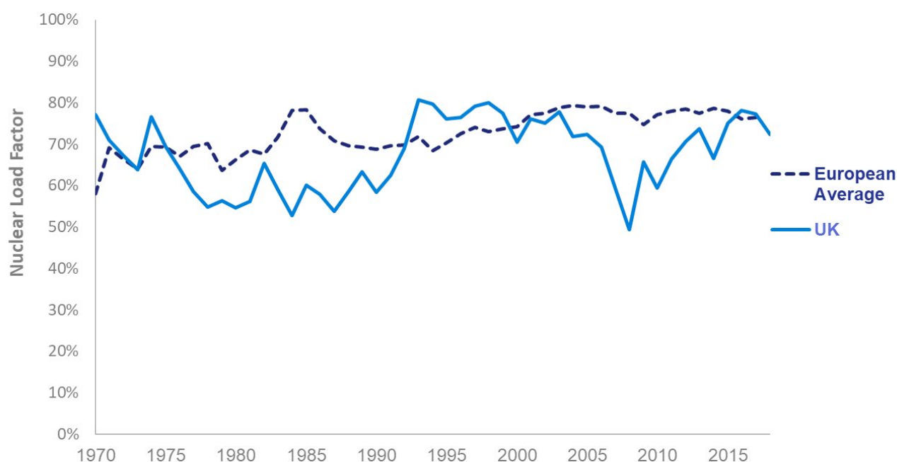
Chart 3: Annual nuclear load factors for the UK 6,7 and Europe 8 , 1970-2018
