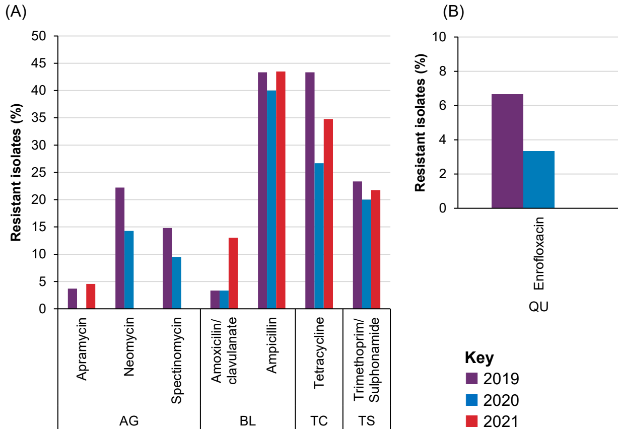
Figure 4.12: Resistance to non-HP-CIAs (A) and HP-CIAs (B) of Escherichia coli isolates from adult cows (n=22 to 23 in 2021). Note scale differs between graphs.
