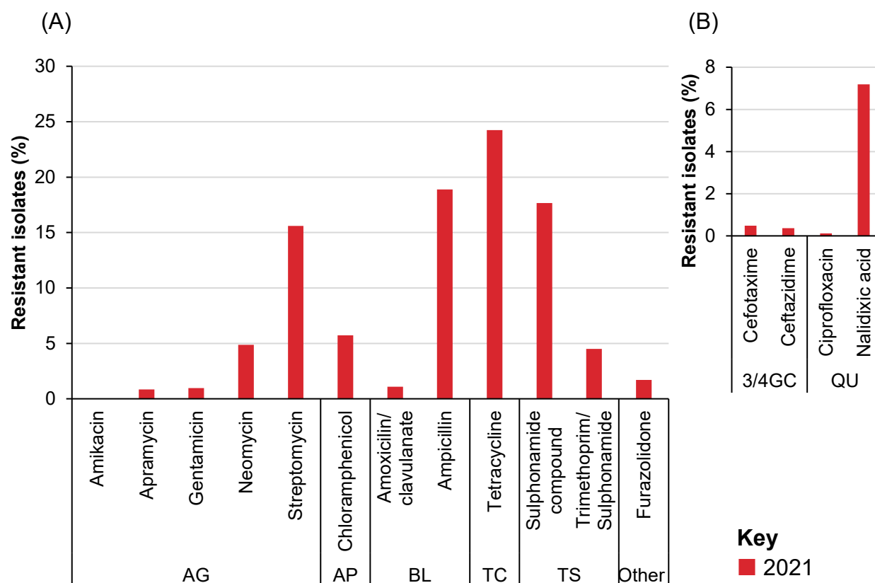
Figure 4.28: Resistance to non-HP-CIAs (A) and HP-CIAs (B) of Salmonella isolates from dogs in 2021. Note scale differs between graphs.
