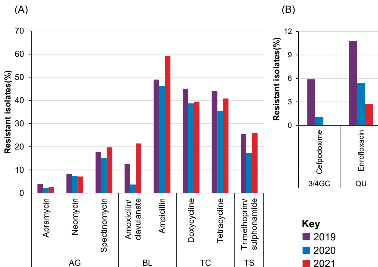
Figure 4.20: Resistance to non-HP-CIAs (A) and HP-CIAs (B) of Escherichia coli isolates from chickens (all ages; n=56 to 147 in 2021). Note scale differs between graphs.
