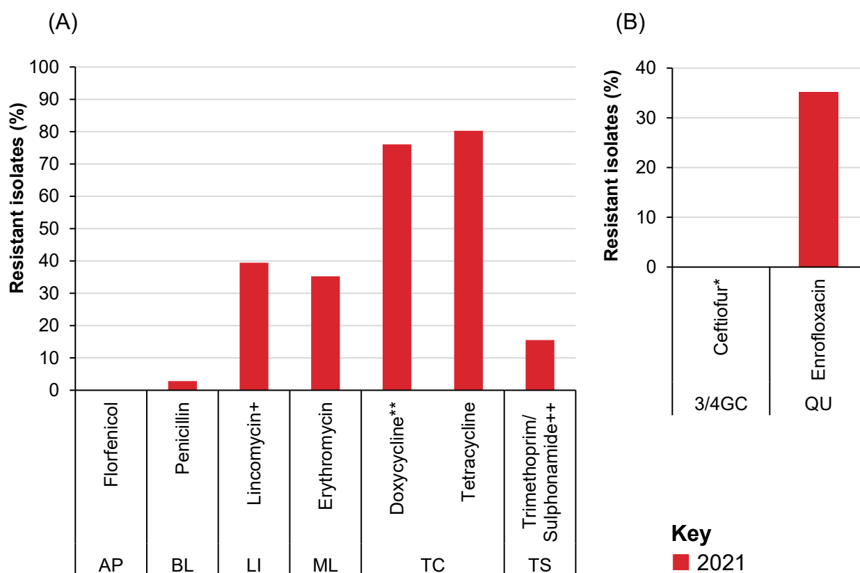
Figure 4.8: Antibiotic resistant of Streptococcus suis isolates from pigs (n=71) interpreted using CLSI veterinary breakpoints unless indicated otherwise.
