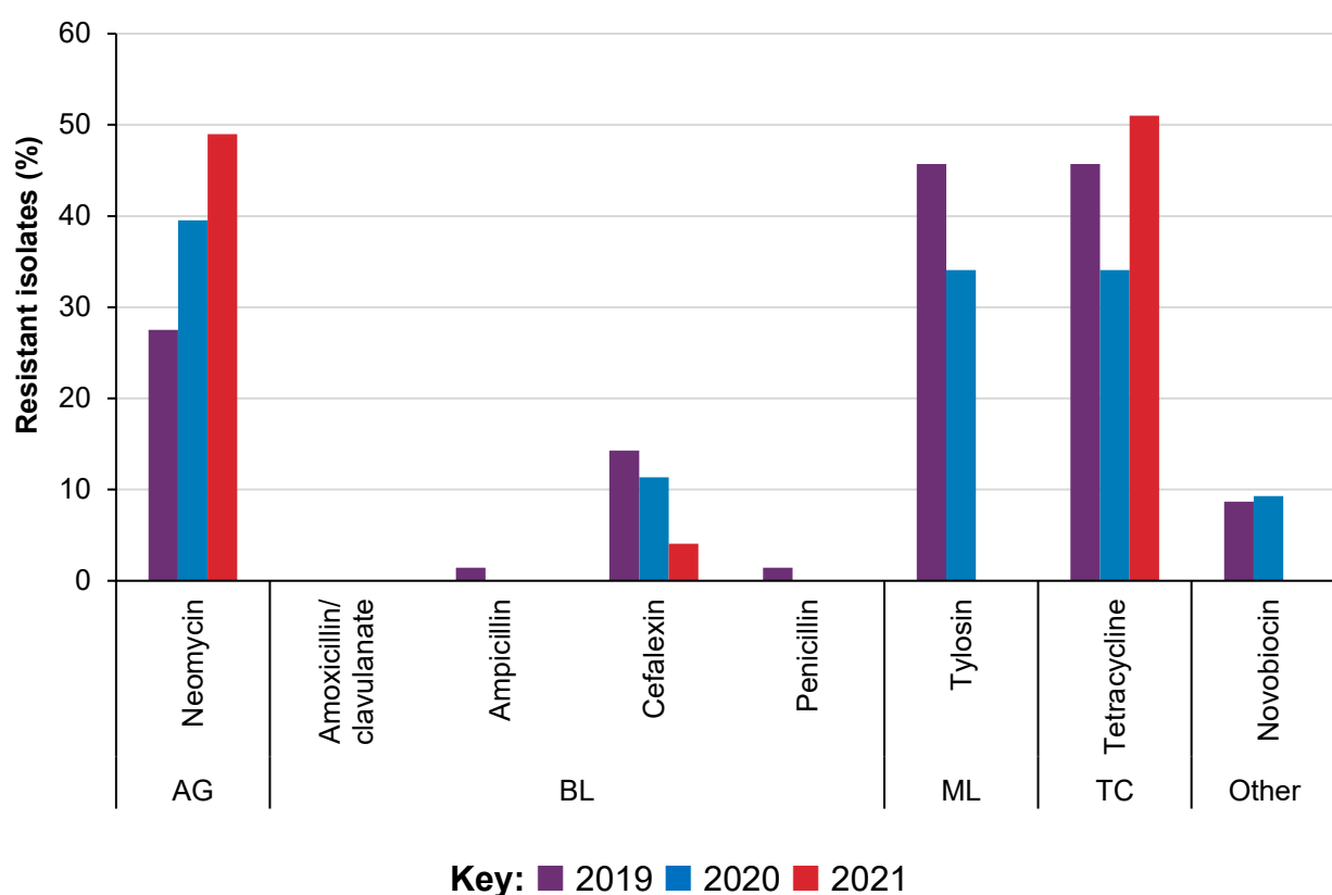
Figure 4.5: Antibiotic resistance of Streptococcus uberis isolated from mastitis samples from cattle (n=49 in 2021) in England and Wales.
