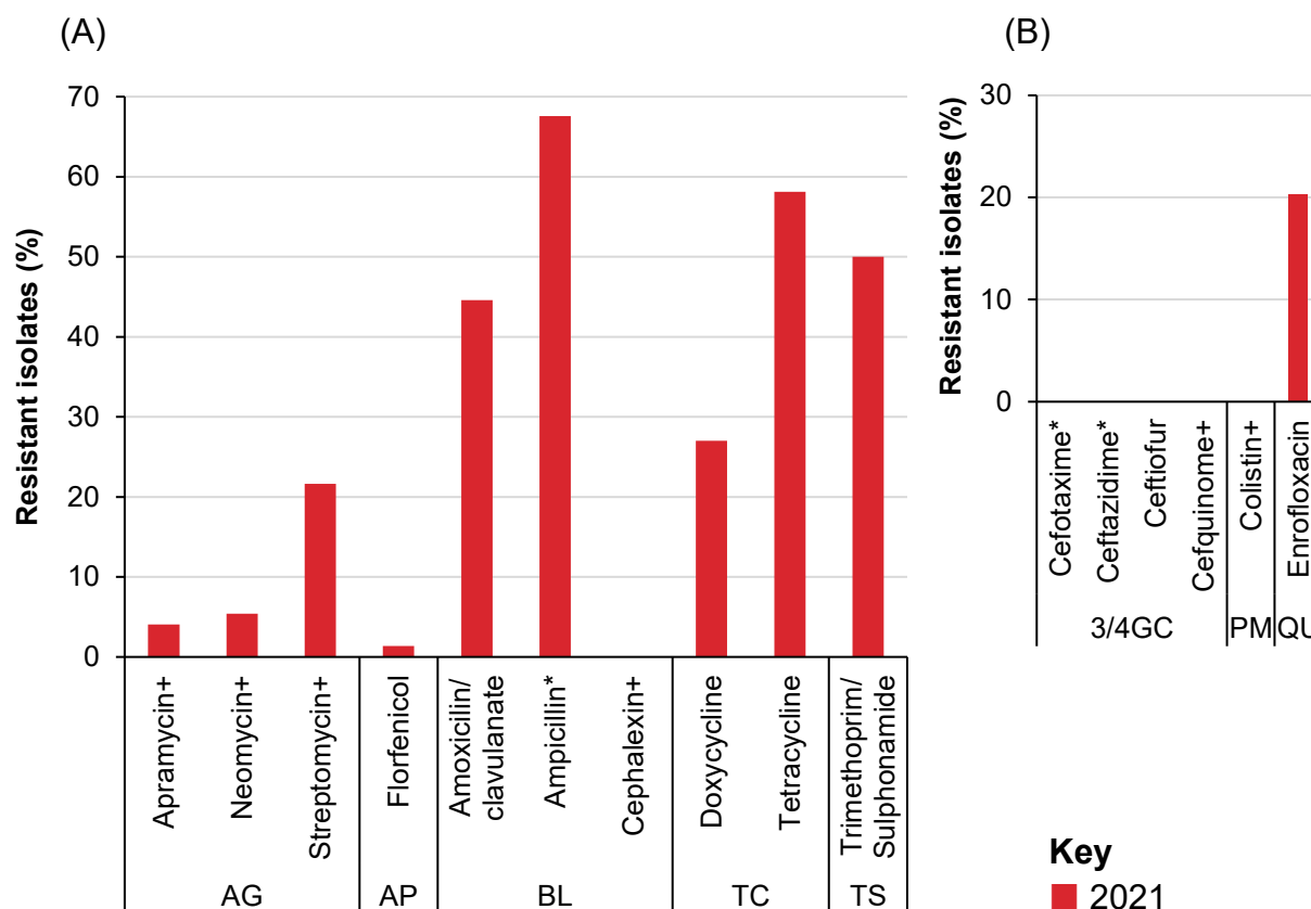
Figure 4.19: Antibiotic resistant isolates of Escherichia coli isolates from poultry (n=74) interpreted using CLSI veterinary breakpoints unless indicated otherwise.
