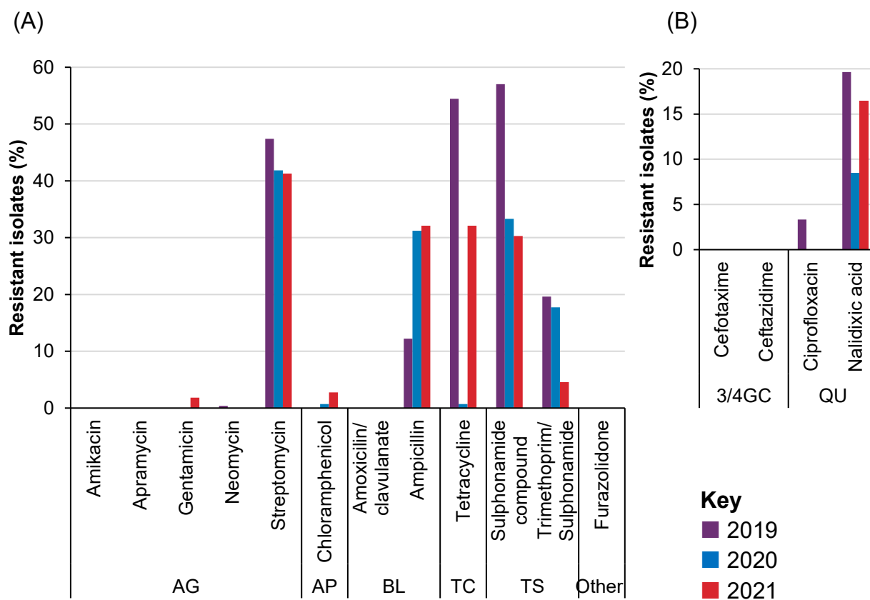
Figure 4.26: Resistance to non-HP-CIAs (A) and HP-CIAs (B) of Salmonella isolates from turkeys (n=109 in 2021) . Note scale differs between graphs.
