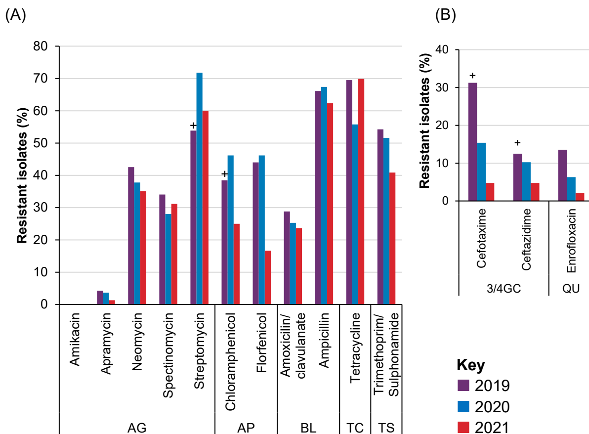
Figure 4.11: Resistance to non-HP-CIAs (A) and HP-CIAs (B) of Escherichia coli isolates from pre-weaned calves (n=20 to 93 in 2021). Note scale differs between graphs.
