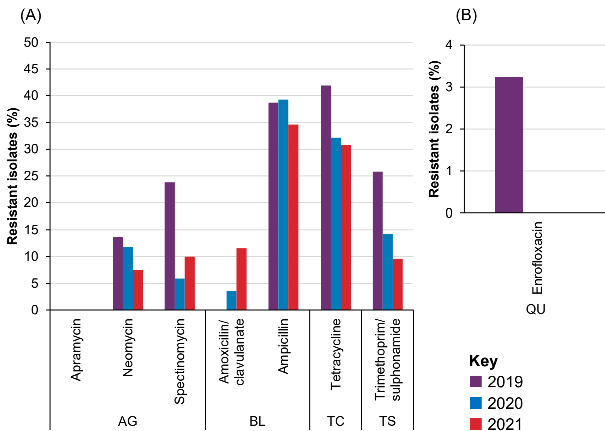
Figure 4.18: Resistance to non-HP-CIAs (A) and HP-CIAs (B) of Escherichia coli isolates from adult sheep (n=40 to 52 in 2021). Note scale differs between graphs.
