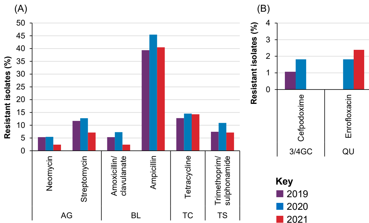
Figure 4.4: Resistance to non-HP-CIAs (A) and HP-CIAs (B) of Escherichia coli isolated from mastitis samples from cattle (n=42 in 2021) in England and Wales. Note scale differs between graphs.
