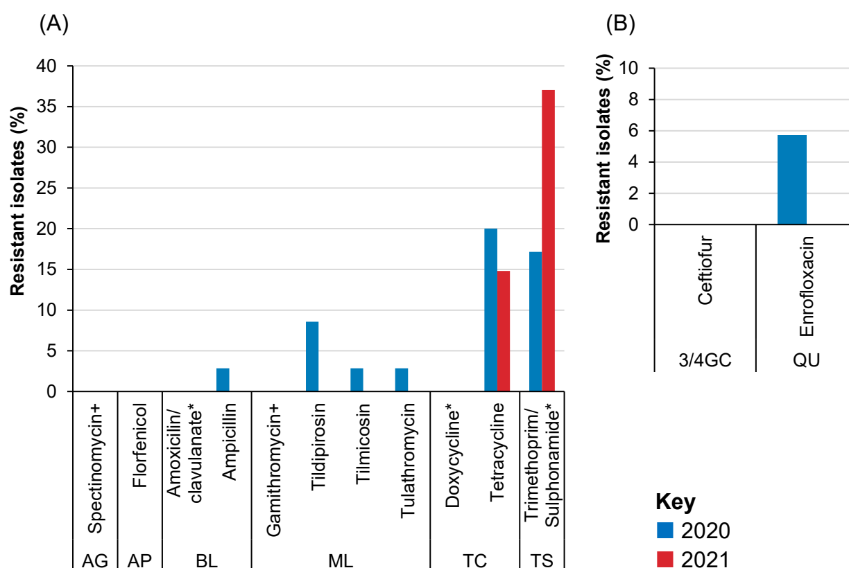
Figure 4.3: Antibiotic resistant of Pasteurella multocida isolates from respiratory infections of pigs (n=27 in 2021) interpreted using CLSI veterinary breakpoints unless indicated otherwise.
