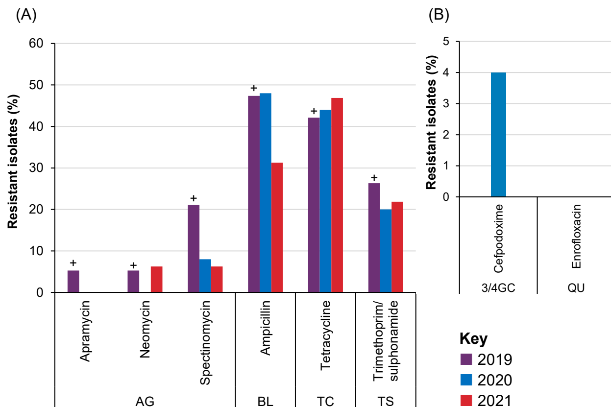
Figure 4.15: Resistance to non-HP-CIAs (A) and HP-CIAs (B) of Escherichia coli isolates from adult pigs (n=32 in 2021). Note scale differs between graphs.
