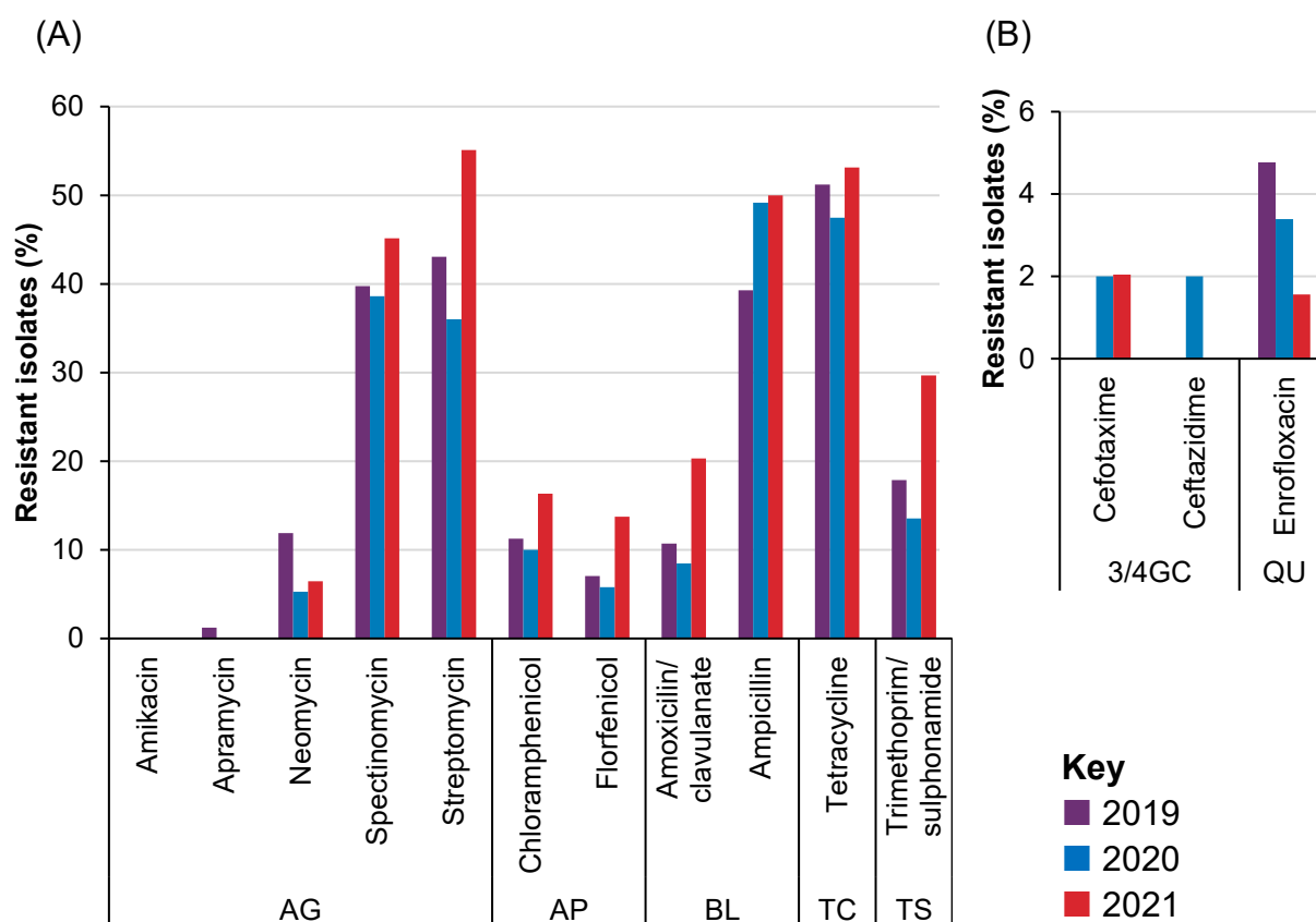
Figure 4.16: Resistance to non-HP-CIAs (A) and HP-CIAs (B) of Escherichia coli isolates from neonatal lambs (n=49 to 64 in 2021). Note scale differs between graphs.
