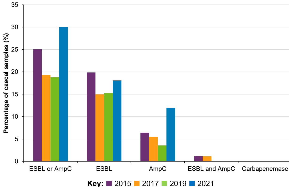
Figure 3.2: ESBL-/AmpC- and carbapenemase producing Escherichia coli cultured on selective agars, from caecal samples from healthy pigs at slaughter in the UK.
